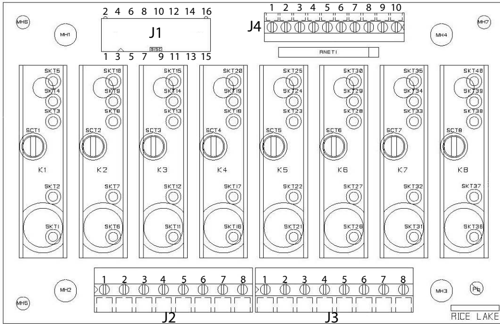
Figure 1. 8-Channel Relay Board
